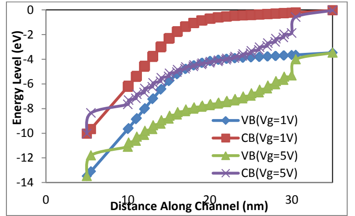
Fig. 3 - Valence and Conduction Band (Variation of V_g from 1 V to 5 V) with V_d = 10\text{V}
