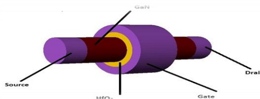
Fig. 1 - 3D structure of the device
