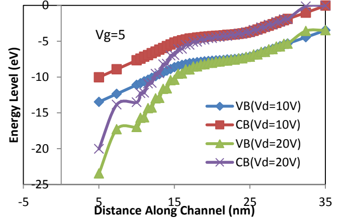
Fig. 2 - Valence and Conduction Band (Variation of V_d from 10 V to 20 V) with V_g = 5\text{V}
