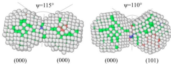
Fig. 4 – Comparison of dihedral angles in the Cu_{381} - Cu_{381} system for different lattice orientations in one of the nanoparticles. Initial distance between nanoparticles, 0.3 nm. Green, blue, and red atoms correspond to fcc, bcc, and hcp lattices, respectively
