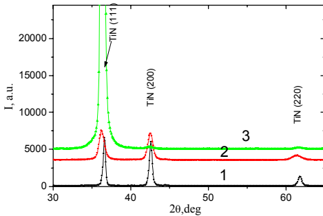
Fig. 3 - Plots of the diffraction spectra of titanium nitride coatings with high-voltage pulses and bias – 5 V (curve 1), –40 (curve 2) and –230 (curve 3)
