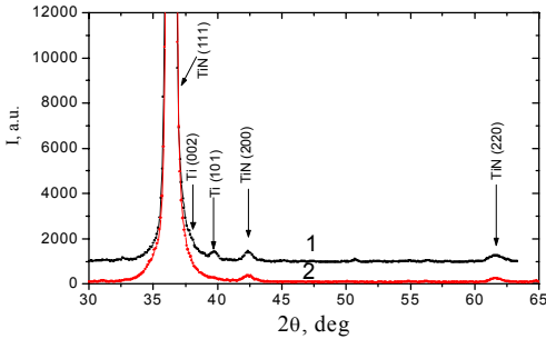
Fig. 2 - Plots of the diffraction spectra of titanium nitride coatings for U_s = -230 without high-voltage pulses (curve 1), with high-voltage pulses (curve 2).
