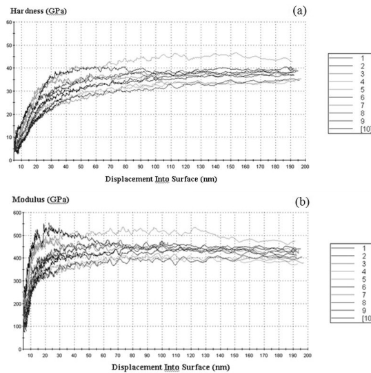
Figure 30. Curves for hardness H (a) and elasticity modulus E (b) obtained for the sample Ti-N-Cr/Ni-Cr-B-Si-Fe. The calculation results for H and E are presented in the Table 10.
