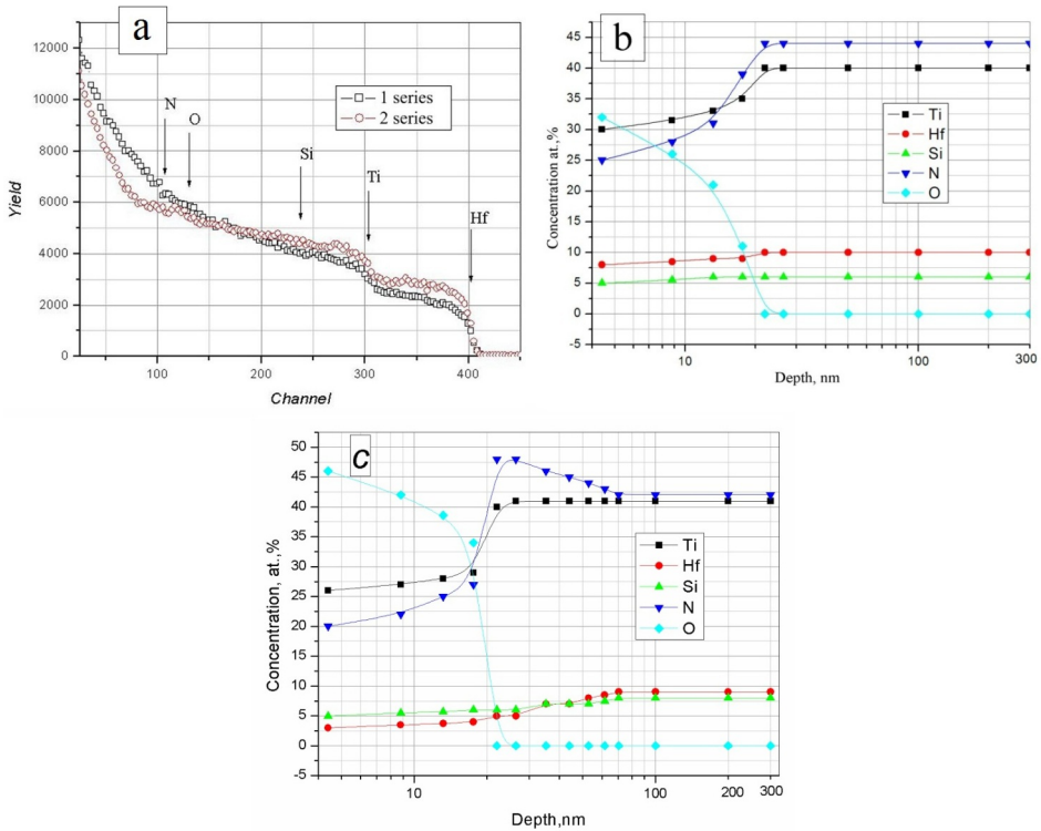
Figure 12. a) RBS spectra of He + with 1,3 MeV energy, obtained from steel sample with Ti-Hf-Si-N film: curve 1-potential 100V, p=0,6 Pa, curve 2 - potential 200V, p=0,7 Pa. (b) The depth profiles of elements in the Ti-Hf-Si-N coating, obtained from RBS spectrums (Figure 12a). Considering that atomic density of layer is close to atomic density of titanium nitride. (c) The depth profiles in the Ti-Hf-Si-N coating obtained from spectrums (2) on Figure 12a (mode 2).
