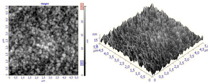
Figure 4. Surface morphology of coatings on base (Zr-Ti-Si)N with U = -150\text{V} , P = 0,8 Pa.
