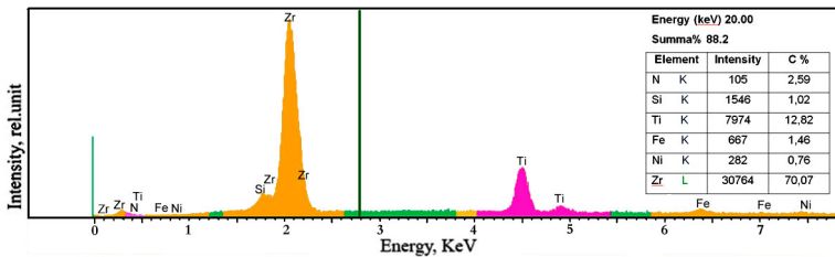
Figure 8. Data of microanalysis for point of Zr-Ti-Si-N (Ti≈12%) nanocomposite coating surface. (fifth series)
