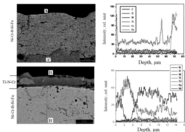
Figure 25. a) Scanning electron microscopy images for the cross-section (A-A') and distribution of the characteristic X-ray element emission over this cross-section (A-A') in a combined nanocomposite coating (a thick coating was melted by a plasma jet). (b) Scanning electron microscopy images for the cross-section and distribution of the characteristic X-ray element emission along the cross-section (B-B') in the coating on the base of (Ti, Cr)N solid solution. The thin coating was deposited on the thick one of Ni-Cr-B-Si-Fe(W) and melted by a plasma jet.
