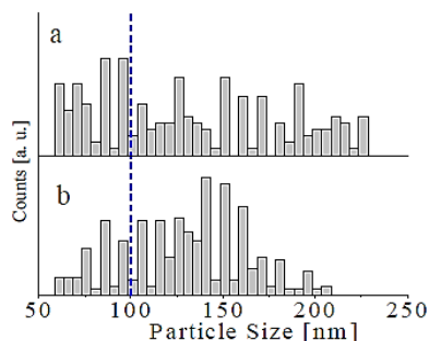
Fig. 2 – Size distributions of silicon nanoparticles prepared by the picosecond laser ablation in de-ionized water (a) with and (b) without applying the additional continuous laser (vertical lines at 100 nm should facilitate comparison).
