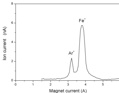
Fig. 9 - Mass-spectrum of ion beam source with a Fe target. U_i = 1.08 kV, I_i = 60 mA, p = 40 Pa, I_s = 12 \mu A
