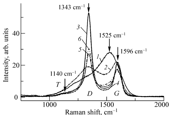
1 – initial DLC film; 2–6 – treated DLC films: 2 – laser fluence 0.4\text{ J/cm}^2 , 3 – 1\text{ J/cm}^2 , 4 – 2.3\text{ J/cm}^2 , 5 – 3.5\text{ J/cm}^2 , 6 – 7.1\text{ J/cm}^2
