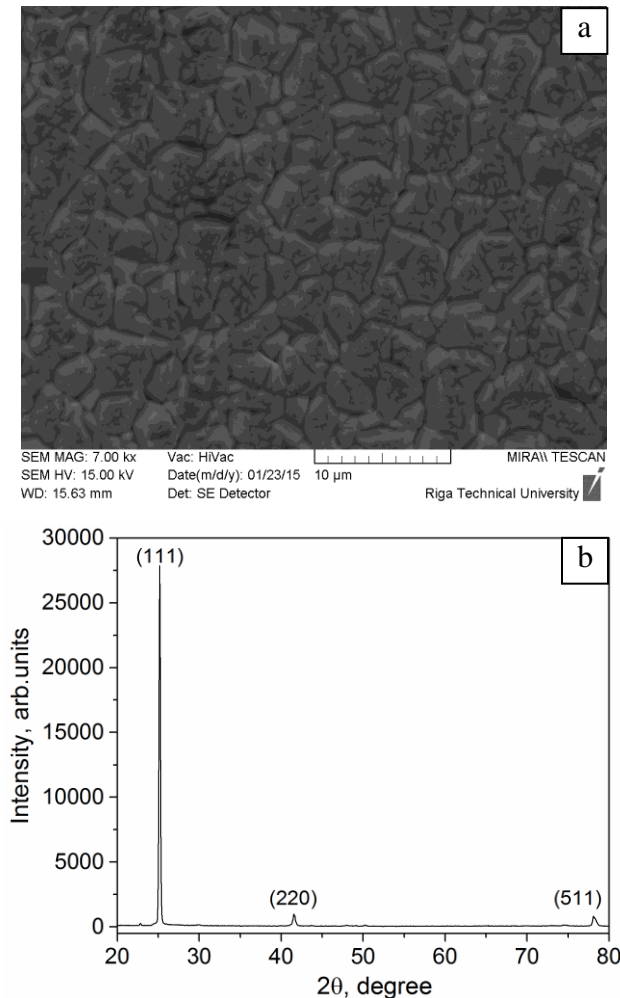
Fig. 1 – Structural properties of CZT film: SEM image of CZT surface (a), XRD pattern (b).
