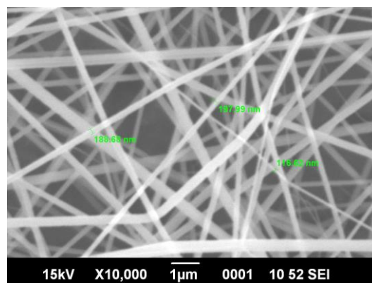
Fig. 2 – SEM images of titanium nano fibers with flow rate 0.5 ml/h
