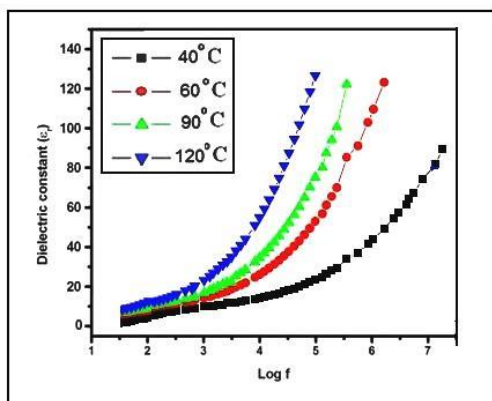
Fig. 6 – Dielectric constant of BaTiO 3 nanoparticles
