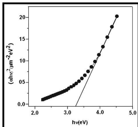
Fig. 5 – Plot of (ah\nu)^2 vs (h\nu)
