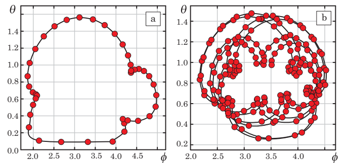
FIG. 6. (Color online) Examples of regular (a) and chaotic (b) trajectories of the magnetic moment driven by the linearly polarized magnetic field. The simulation parameters are \rho = 0 , \tilde{H} = 0 , \alpha = 0.1 , \tilde{\omega} = 0.8 , and \tilde{h} = 0.4 (a) and \tilde{h} = 0.46 (b).
