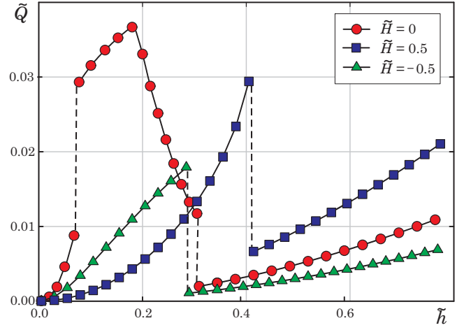
FIG. 5. (Color online) Reduced power loss \tilde{Q} as a function of the reduced amplitude \tilde{h} of circularly polarized magnetic field for different values of the reduced magnetic field \tilde{H} . The parameters \rho , \alpha , and \tilde{\omega} are the same as in Fig. 4.
