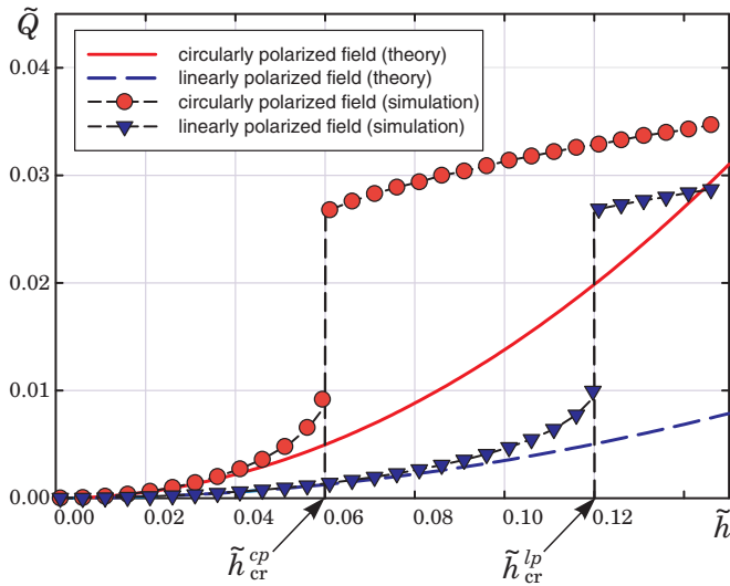
FIG. 2. (Color online) Reduced power loss \tilde{Q} as a function of the reduced amplitude \tilde{h} for circularly ( \rho = +1 ) and linearly ( \rho = 0 ) polarized magnetic fields. The solid and dashed lines represent the theoretical results obtained from Eqs. (3.6) and (3.15), respectively, and the symbols show the numerical results obtained from Eq. (4.1). It is assumed that \sigma = +1 , \alpha = 0.1 , and \tilde{\omega} = 0.8 .
