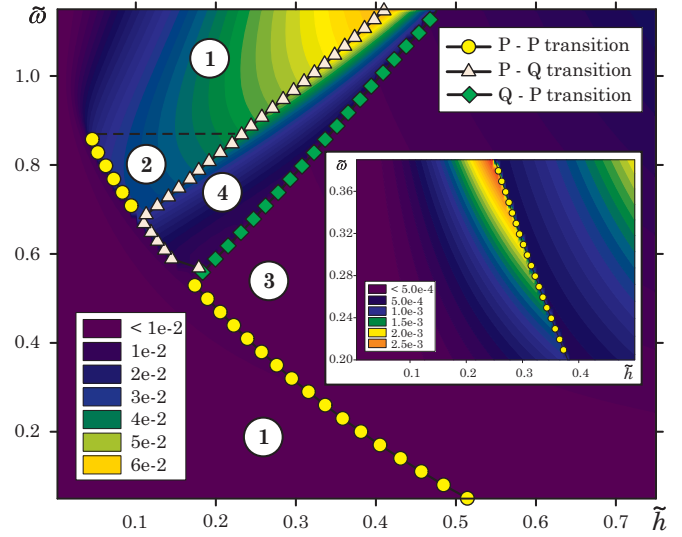
FIG. 3. (Color online) Color map for the reduced power loss \tilde{Q} and the diagram for the steady-state regimes of precession of the magnetic moment driven by the circularly polarized magnetic field. The regions with different periodic regimes of precession are indicated by numbers 1–3, and the region with the quasiperiodic regime of precession by number 4. The numerical results are obtained for \rho = +1 , \tilde{H} = 0 , and \alpha = 0.1 .
