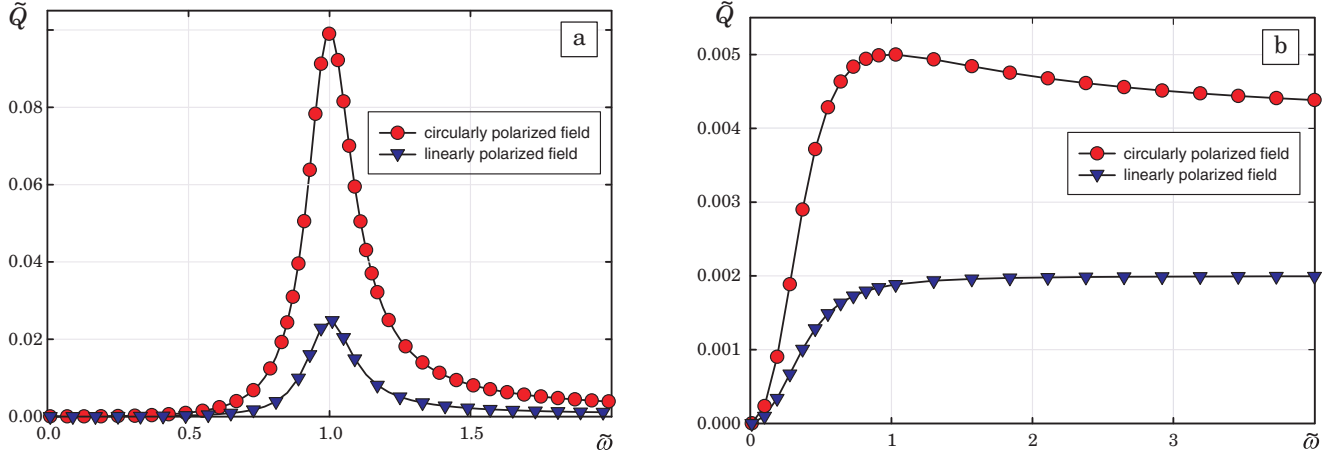
FIG. 1. (Color online) Reduced power loss \tilde{Q} as a function of the reduced frequency \tilde{\omega} in the small amplitude approximation. The parameters used in Eqs. (3.6) and (3.15) are \tilde{h} = 0.1 , \tilde{H} = 0 , \sigma = +1 , \rho = +1 , and \alpha = 0.1 (a) and \alpha = 2 (b).
