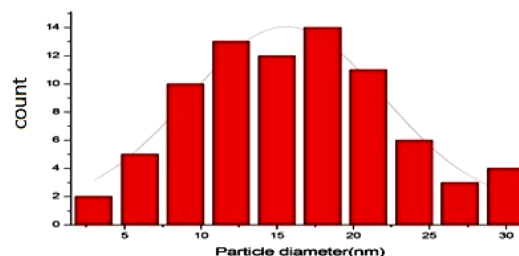
Fig. 1 – Size distribution of nanoparticles generated by Nd:YAG laser (1064 nm, 12 ns, 80 mJ/pulse, 5 Hz, spot size on the target \sim 700 \mu m , 10 min exposure time)
