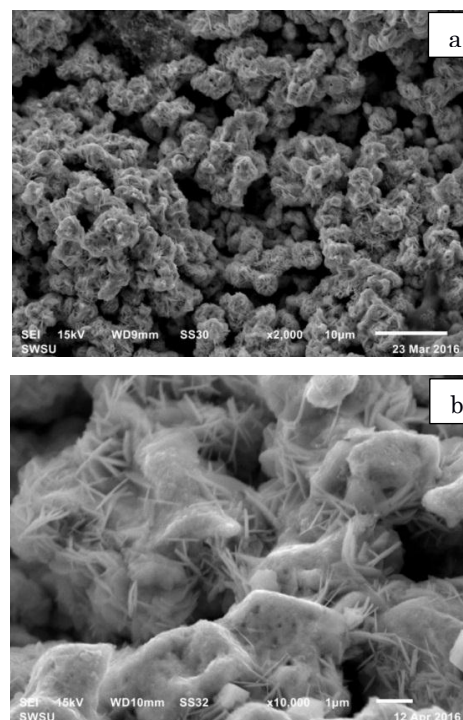
Fig. 3 – Negative active material after a battery testing in the cycling mode at various magnifications
