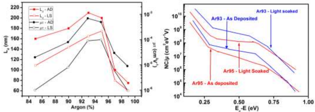
Fig. 1: Evolution of L_p and \mu\tau product with flow variation Fig. 2: DOS data of Ar93 and Ar95 in AD and LS state
