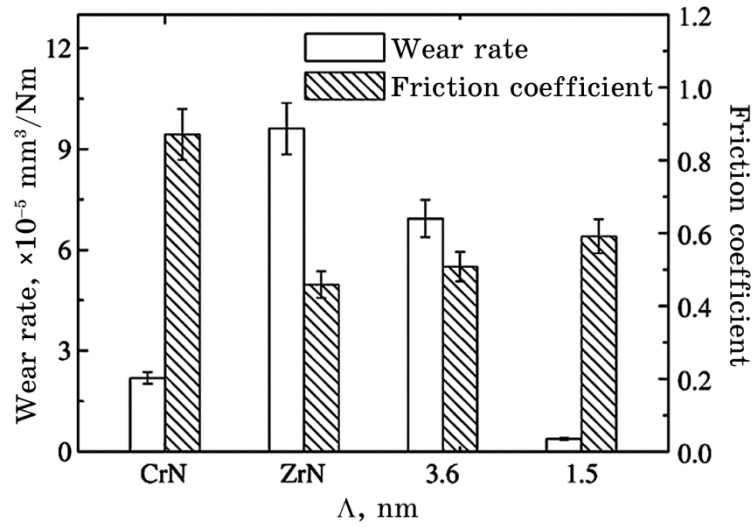
Fig. 13. Wear rate and friction coefficient vs. estimated modulation period \Lambda obtained at P_N = 2.6 \cdot 10^{-1} Pa, U_s = -200 V, T_s = 200^\circ\text{C} for the CrN/ZrN coatings [37].
