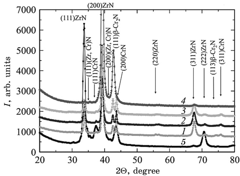
Fig. 7. Regions of diffraction spectra obtained at P_N = 4 \cdot 10^{-3} \text{ Torr} , U_s = -150 \text{ V} , U_i = -800 \text{ V} for coatings with different bilayer thickness: 300 nm (1), 120 nm (2), 80 nm (3), 40 nm (4), and \approx 20 \text{ nm} (5) [31].
