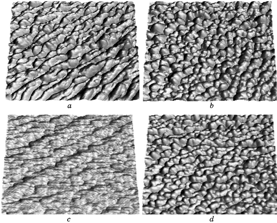
Fig. 4. The 1.0 \times 1.0 \mu\text{m} AFM images of CrN/ZrN coatings with bilayer thickness ( \Lambda ) of 3 \mu\text{m} (a), 375 \mu\text{m} (b), 200 \text{ nm} (c), and 100 \text{ nm} (d) [35].
