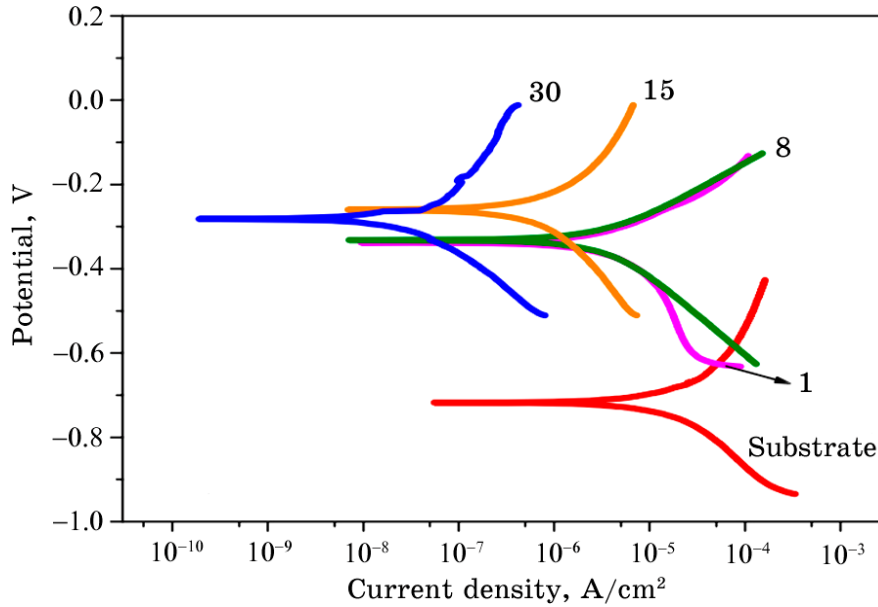
Fig. 11. Tafel polarization curves for CrN/ZrN films with 1, 8, 15, and 30 bilayers [35].
