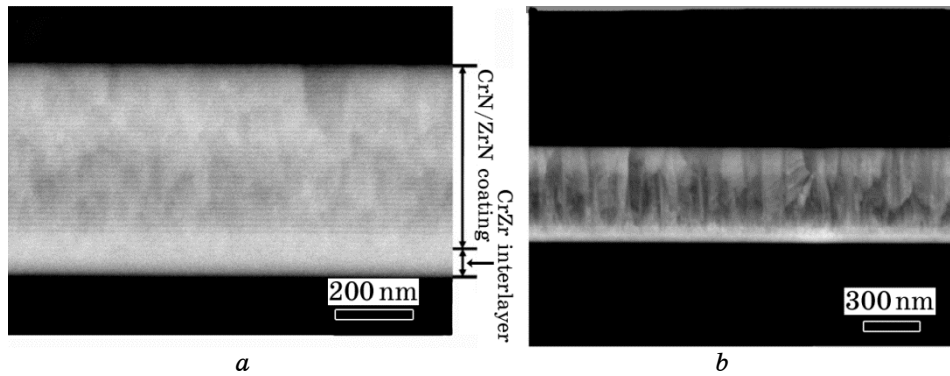
Fig. 2. SEM surface morphologies for the lateral surface of the multilayer CrN/ZrN coatings obtained at P_N = 8.6 \cdot 10^{-1} Pa, T_S = 150^\circ\text{C} , U_S = -100 V with different bilayer thickness ( \Lambda ): 16 nm (a) [32] and 6 nm (b) [33].
