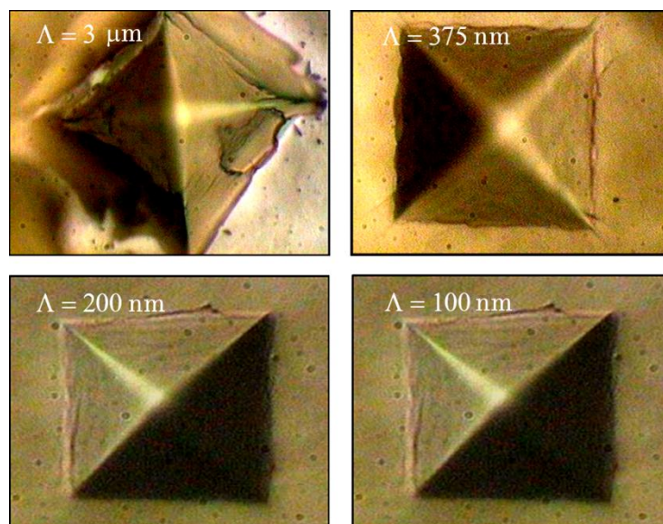
Fig. 15. The AFM micrographs of the Vickers indentation print for the CrN/ZrN coatings obtained on steel substrates via magnetron sputtering at P_N = 0.66 Pa, U_s = -60 V, T_s = 250^\circ\text{C} [35].
