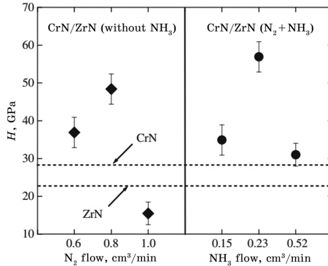
Fig. 10. Nanoindentation hardness ( H ) vs. the flow rate of N_2 and N_2 + NH_3 reaction gases obtained at P_N = 2.8 \cdot 10^{-1} Pa, U_S = -200 V, T_S = 200^\circ C via dc magnetron sputtering of multilayer CrN/ZrN coatings on Si substrates [38].
