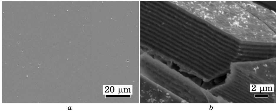
Fig. 1. The scanning electron microscopy (SEM) images of nanocomposite ZrN/CrN coating with a modulation period of 300 nm obtained for surface (a) and fracture (b) at P_N = 4 \cdot 10^{-3} Torr, T_S = 250\text{--}350^\circ\text{C} , U_S = -150 V [30].
