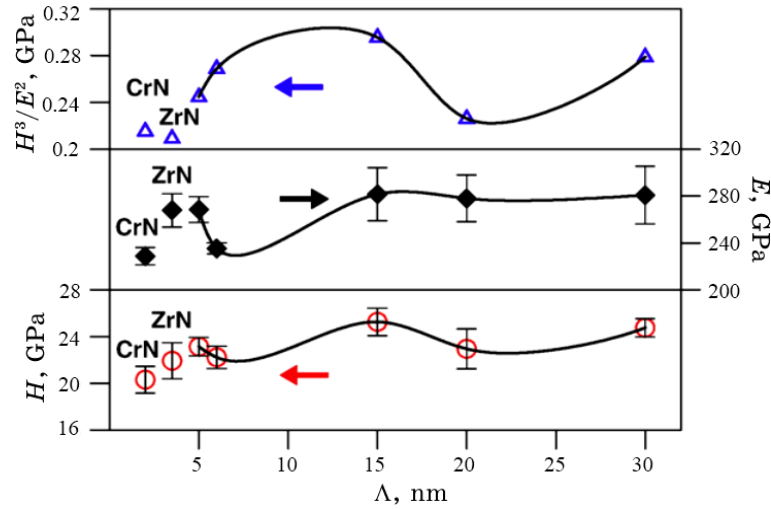
Fig. 9. The hardness ( H ), elastic modulus ( E ), and plastic deformation resistance ( H^3/E^2 ) vs. the bilayer periods ( \Lambda ) for the CrN/ZrN multilayered coatings on Si substrates obtained at P_N = 8.6 \cdot 10^{-1} Pa, U_S = -100 V, T_S = 150^\circ\text{C} via the arc-PVD technique [33].
