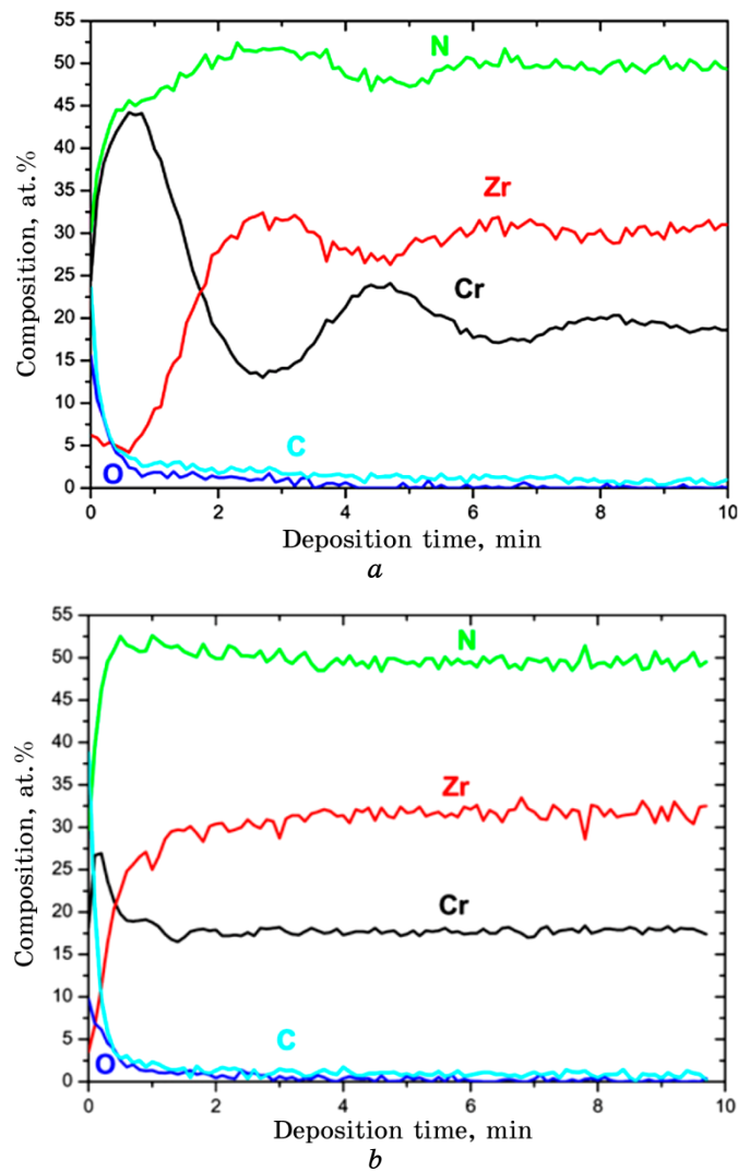
Fig. 5. Composition depth profile for multilayer CrN/ZrN coatings obtained at P_N = 3.3 \cdot 10^{-3} Torr, T_S = 150^\circ\text{C} , U_S = -100 V with different bilayer thickness ( \Lambda ): 7.1 nm (a) and 2.1 nm (b) [36].
