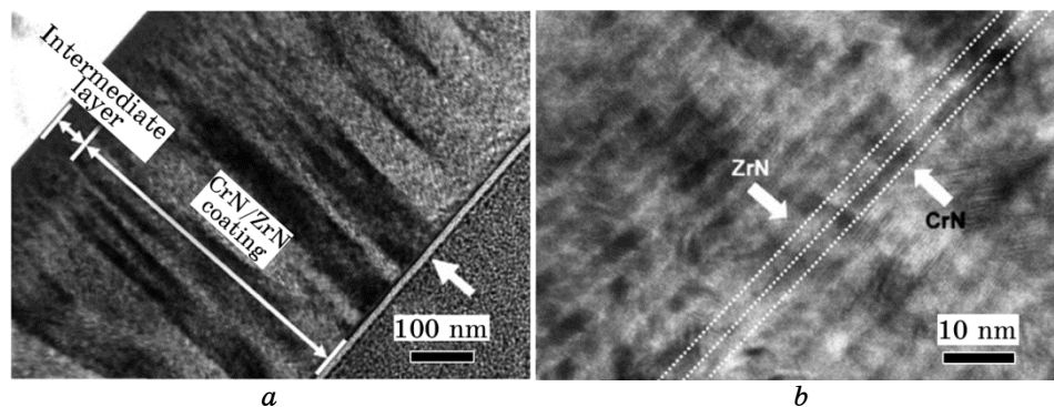
Fig. 3. The cross-sectional transmission electron microscopy (TEM) micrographs of the multilayer CrN/ZrN with bilayer thickness of 5 nm for lower (a) and higher (b) magnifications [33].
