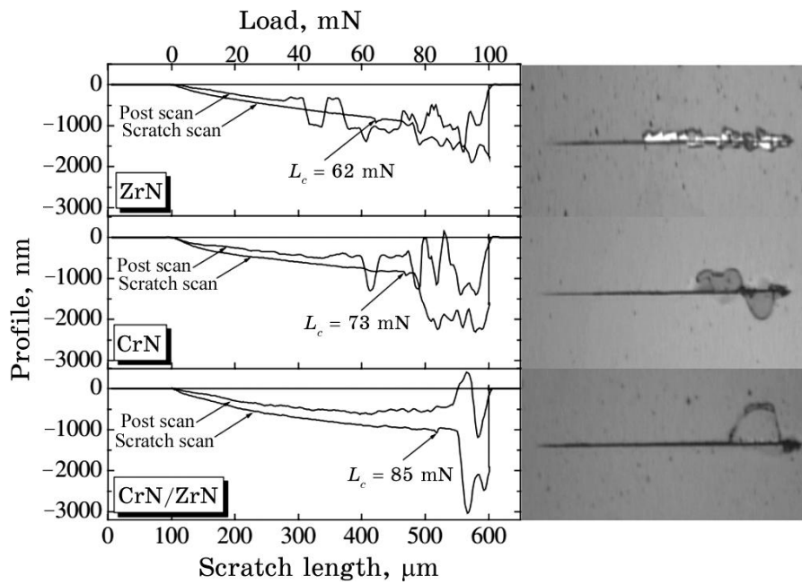
Fig. 14. Surface profiles of the scratch scan and post scan along with the scratch tracks images of the multilayer CrN/ZrN coatings [39].
