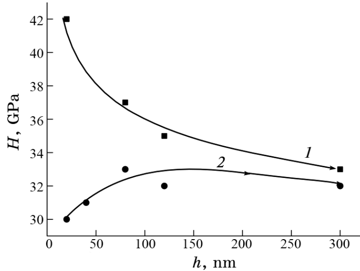
Fig. 8. Dependence of hardness H on the layer thickness h in ZrN/CrN multilayer coating produced at P_N = 4 \cdot 10^{-3} Torr and pulsed stimulation of deposition U_I = -800 V for two cases: without (1) and with application of a constant voltage U_S = -150 V (2) [31].
