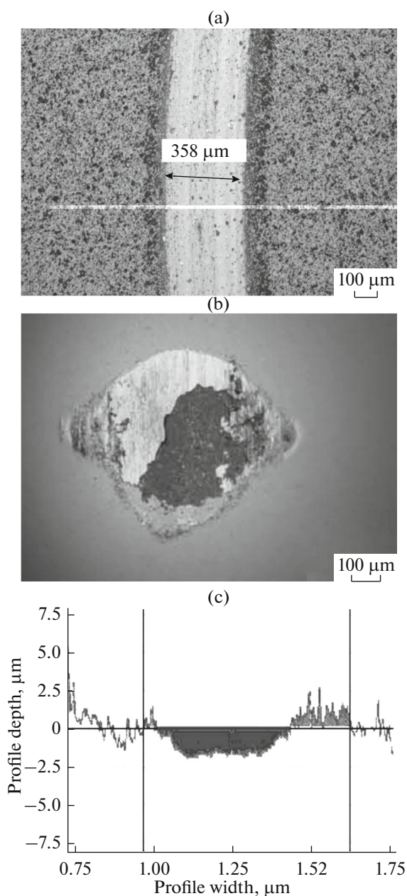
Fig. 6. Wear track on the (a) surface of coating and (b) Al 2 O 3 ball counterbody and (c) profile of the wear groove of the coating after testing of (TiAlSiY)N coating (batch 1).
