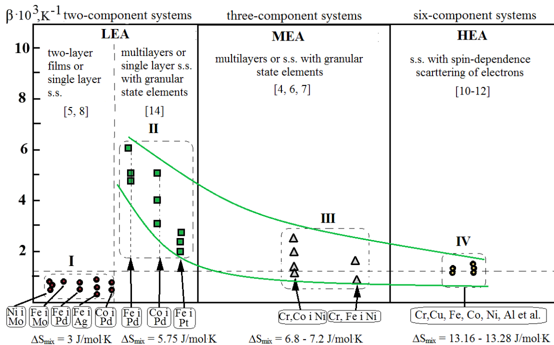
Fig. 1 – Correlation between TCR and \Delta S_{\text{mix}} for films with different entropy degree
