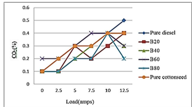
Figure 9 – Load vs. CO 2
