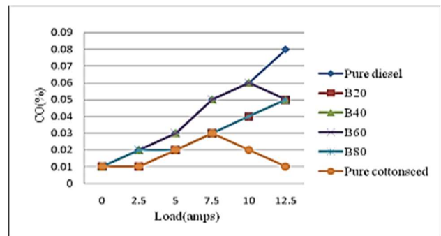
Figure 10 – Load vs. CO
