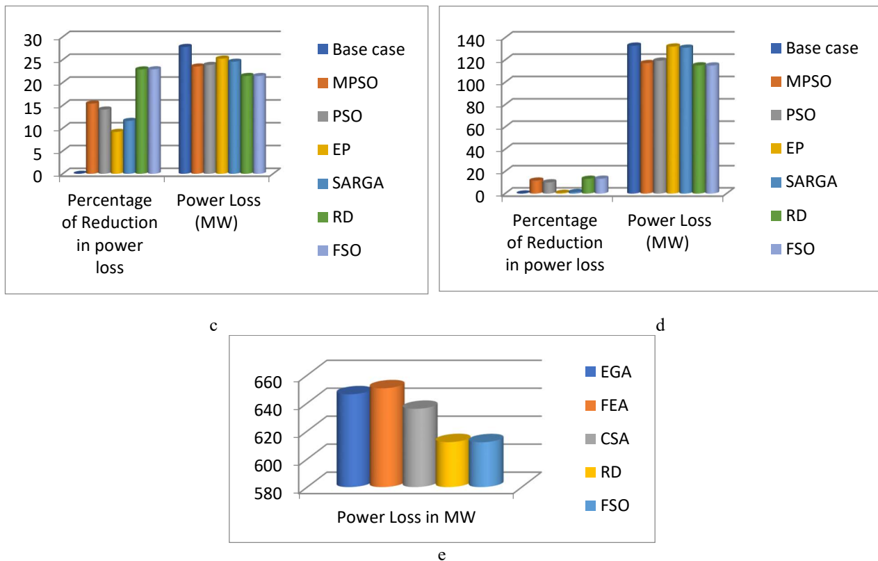
Figure 1 – Comparison of power losses: IEEE14 bus system (a); IEEE 30 bus system (b); IEEE 57 bus system (c); IEEE 118 bus system (d); IEEE 300 bus system (e)
