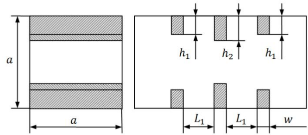
Fig. 1 – Inner structure of a waveguide polarizer with 3 irises
