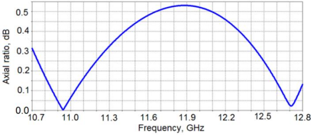
Fig. 9 – Axial ratio vs. frequency for a polarizer with 4 irises
