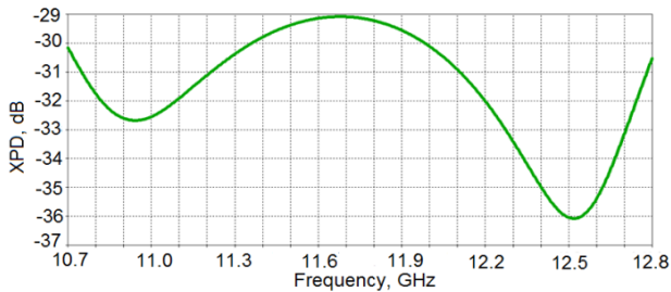
Fig. 5 – XPD vs. frequency for a polarizer with 3 irises
