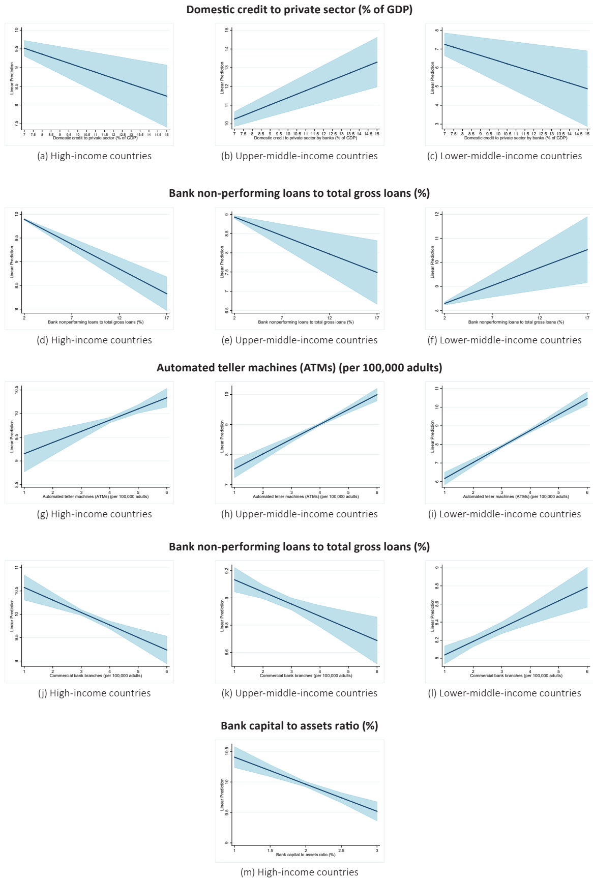
Figure A1. Predictive margins with 95% for independent variable by groups
