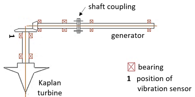
Figure 5. Schematic representation of the Kaplan turbine assembly
