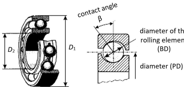
Figure 4. Elements of a bearing
