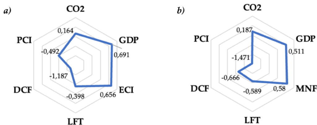
Figure 6. Results for (a) fixed- and (b) random-effects models.
