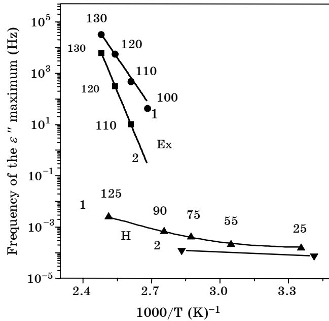
Fig. 3 – Dependence of the experimentally measured ( Ex ) and calculated by Hamon's method ( H ) frequency corresponded to the maximum of the dielectric losses of the PS/DR1 samples (1) and pure PS (2) at different temperatures (shown by figures near curves). Results of calculations by Arrhenius formula are shown by solid lines.
