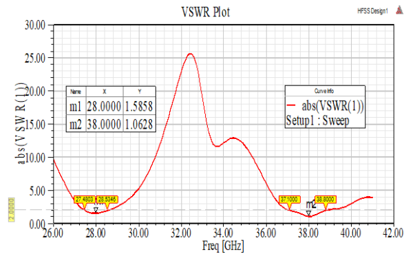
Fig. 6 – VSWR Plot
