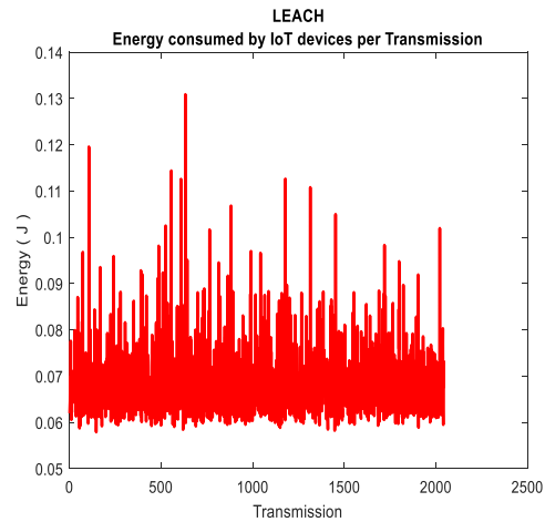
Fig. 4 – Energy consumed
