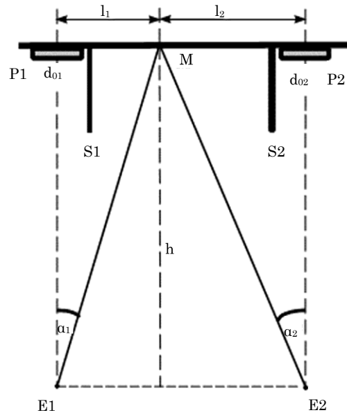
Fig. 1 – Geometry of the «substrate-evaporators» system for calculating the concentration of the alloy components: S1, S2 – screens; E1, E2 – evaporators; P1, P2 – glass plates "witnesses" of thickness
