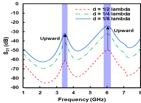
Fig. 6 shows the simulation results from S_{21} from the distance iteration ( d ) where the proposed distance is in the range of 1/2\lambda - 1/8\lambda . The simulation results show that the distance between the antennas greatly affects the S_{21} of the MIMO antenna where low mutual coupling with S_{21} of -61.10 dB and -50.06 dB for f_{r1} and f_{r2} are obtained when d = 1/2\lambda .
