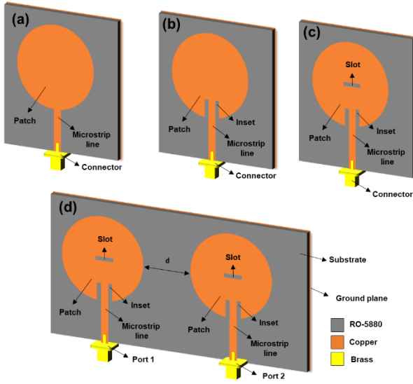
Fig. 1 – Development model of Dual-Band MIMO CPMA, (a) CPMA, (b) CPMA with inset feed, (c) CPMA with inset and slot, (d) CPMA with MIMO configuration
