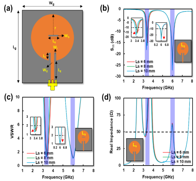
Fig. 4 – (a) Dimension of CPMA with inset feed and slot, (b) S_{11} of CPMA with inset feed and slot, (c) VSWR of CPMA with inset feed and slot, (d) real impedance of CPMA with inset feed and slot
