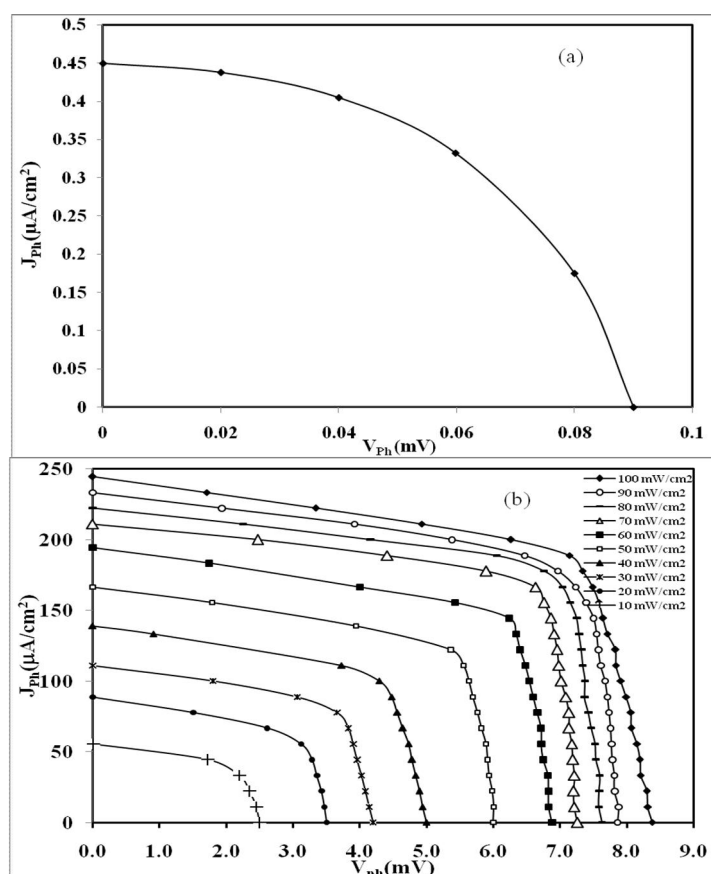
Fig. 1 – The dark J_{ph} \rightarrow V_{ph} characteristics of MoSe 2 /polyaniline solar cell (a) and J_{ph} \rightarrow V_{ph} characteristics of MoSe 2 /Polyaniline solar cell at different intensities of illuminations (b)
