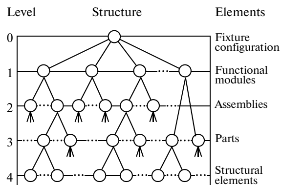
Fig. 1. Hierarchical structure of fixture.
