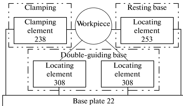
Fig. 8. Graphical model of optimal fixture configuration.
