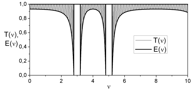
Fig. 2 - Spectral dependencies T(\nu) and E(\nu) of the filter (8) at n_A = 2.3 , n_X = 1.83 , n_B = 1.67 , n_Y = 2.1 , n_S = 1.5 , N = 10
