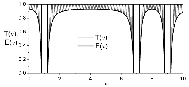
Fig. 1 - Spectral dependencies T(\nu) and E(\nu) of the filter (8) at n_A = 2.3 , n_X = 2.89 , n_B = 1.67 , n_Y = 1.338 , n_S = 1.5 , N = 10
