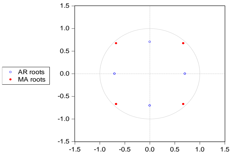
Figure 10. Unit circle
