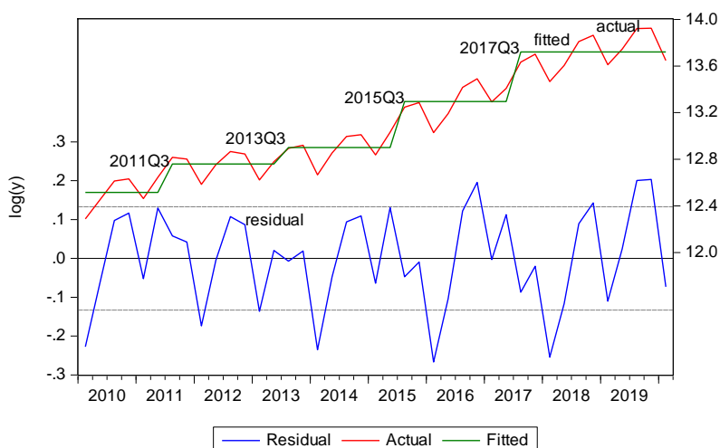
Figure 3. Structural breaks
