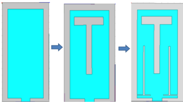
Fig. 2 – Evolution of patch
