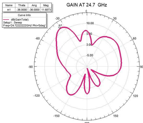
Fig. 14 – Gain at 24.7 GHz
