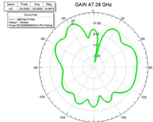
Fig. 15 – Gain at 28 GHz
