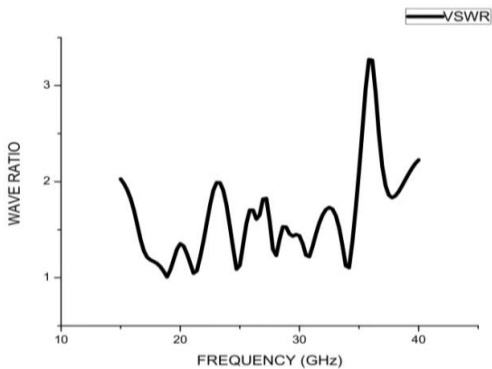
Fig. 11 – Wave Ratio of proposed radiator
