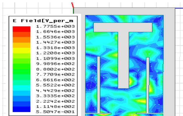
Fig. 8 – Surface Current at 24.7 GHz
