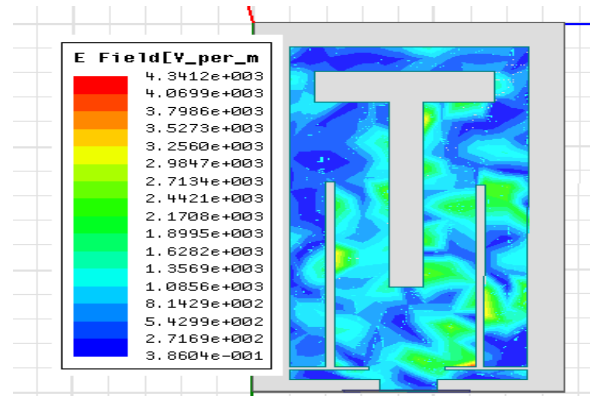
Fig. 9 – Surface Current at 28 GHz
